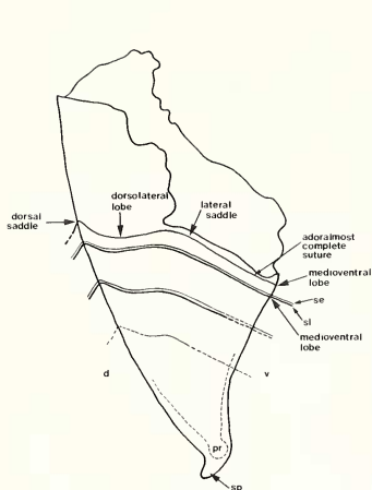
TEXT-FIG. 10. Camera-lucida drawing of the suture lines, septal lines, and protoconch of the holotype of Vectibelus vectensis (Spath, 1939) reproduced in Pl. 24, fig. 1A-K, \times 12 . Lateral view with the addition of the parts of dorsal saddle and ventral lobe not visible in this aspect. All suture and septal lines and protoconch somewhat schematic as they were obscured by the thin guard. The protoconch was drawn using very strong spot light. Abbreviations: sl—suture line; se—septal line; pr—protoconch; sp—apical spine of the guard; d—dorsum; v—venter.
